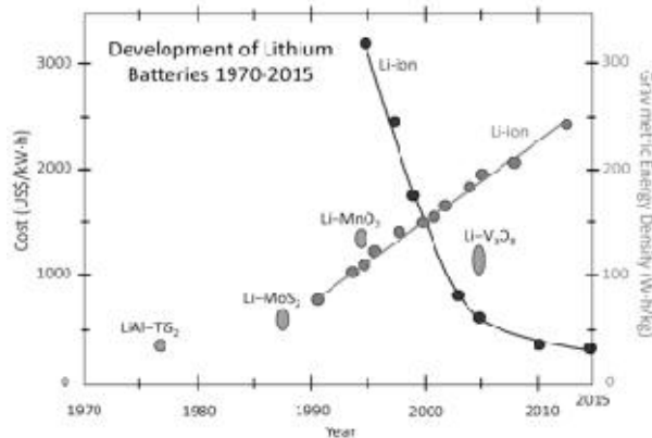
Figure 1. Cost Trend for Lithium-Ion Batteries (Crabtree, et al., 2015, p. 1073)
